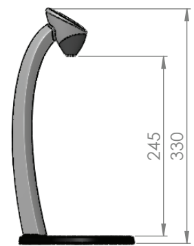
VI Counter top Tap with integral drip tray
