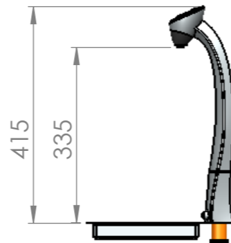
Vi Counter Top Tap with recessed drip tray
